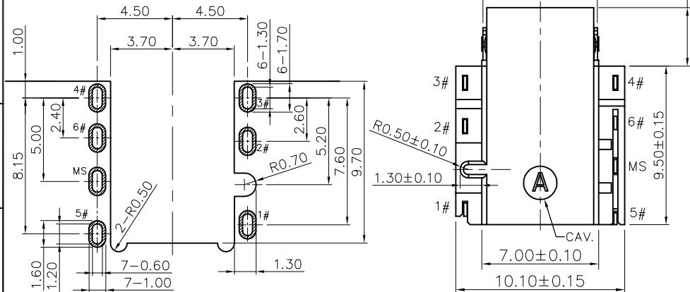
RECOMMAND P.C.B LAYOUT TOLERANCE: ±0.05
