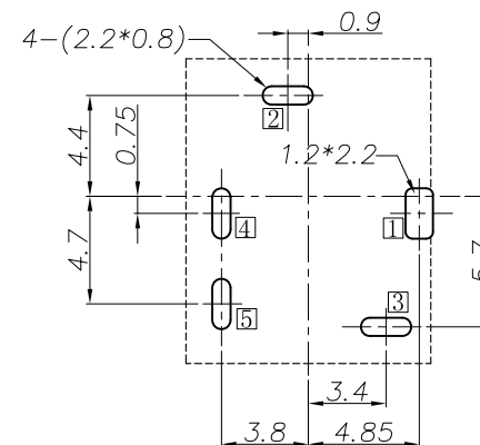
RECOMMENDED P.C.B. LAYOUT UNSPECIFIED TOLERANCE: ±0.05 (COPPER-SIDED VIEW)
