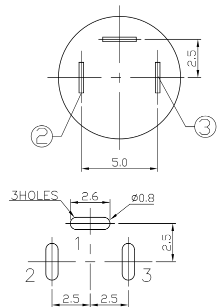
T:1.6 Dimensions of PC board holes Tolerance : ±0.05(Printed-Top view)
